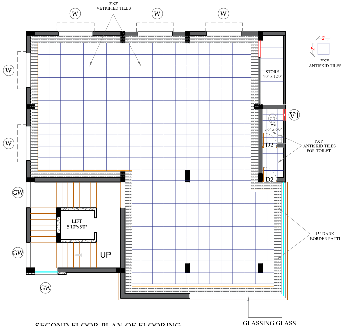
SECOND FLOOR PLAN OF FLOORING
