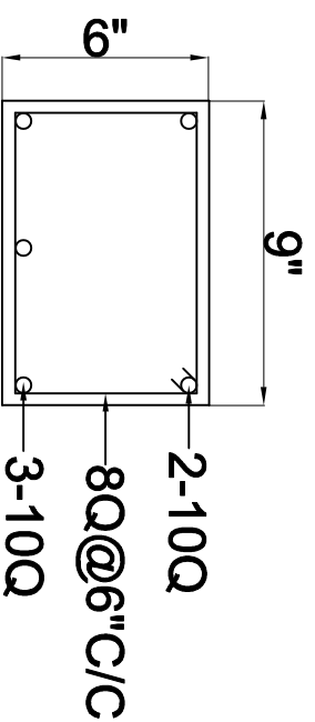
DET-L2(upto 6'0" wide opening)
