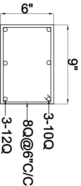
DET-L1(for 6'0" to 9'0" wide opening)
